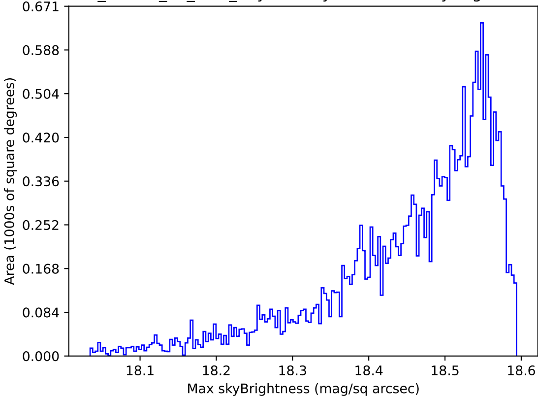
ddf_loaded_fl1_v3.4_10yrs Yr 1 y band: Max skyBrightness
