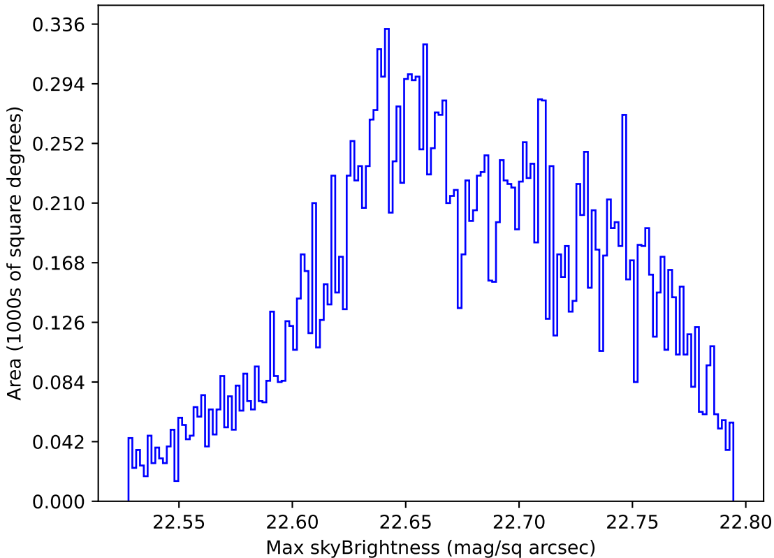
ddf_loaded_fl1_v3.4_10yrs Yr 1 u band: Max skyBrightness
