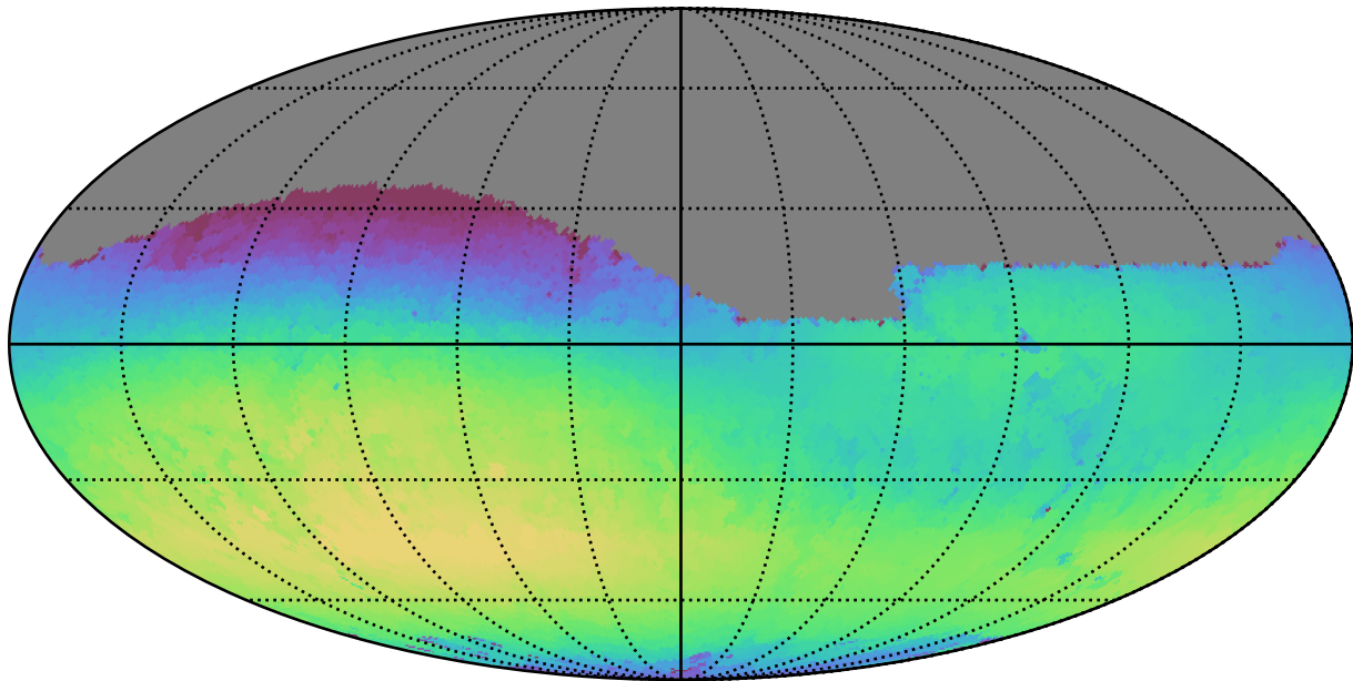
ddf_loaded_fl1_v3.4_10yrs Yr1 r band: Max skyBrightness
