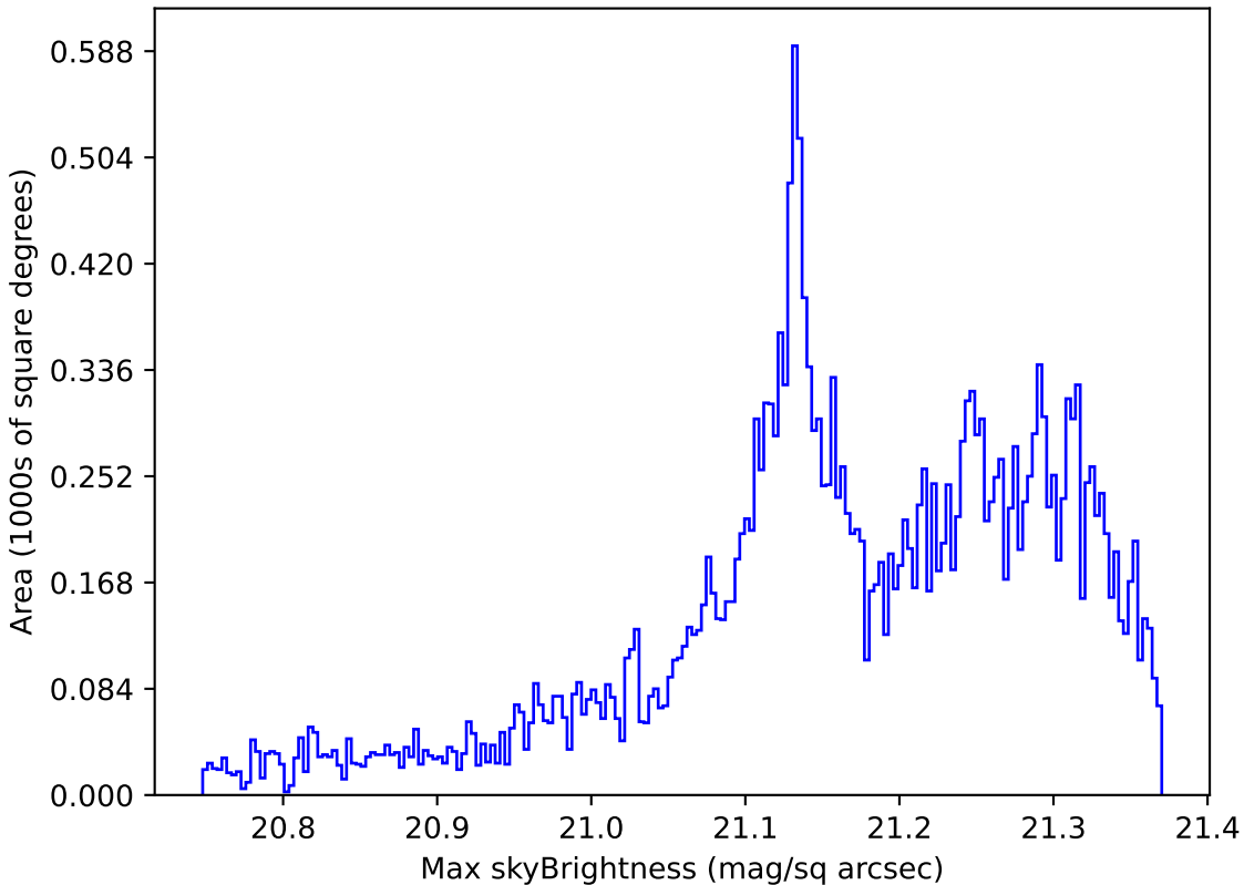
ddf_loaded_fl1_v3.4_10yrs Yr 1 r band: Max skyBrightness
