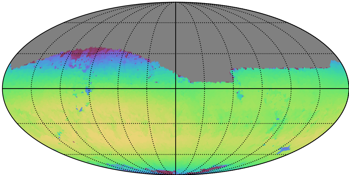
ddf_loaded_fl1_v3.4_10yrs Yr 1 i band: Max skyBrightness
