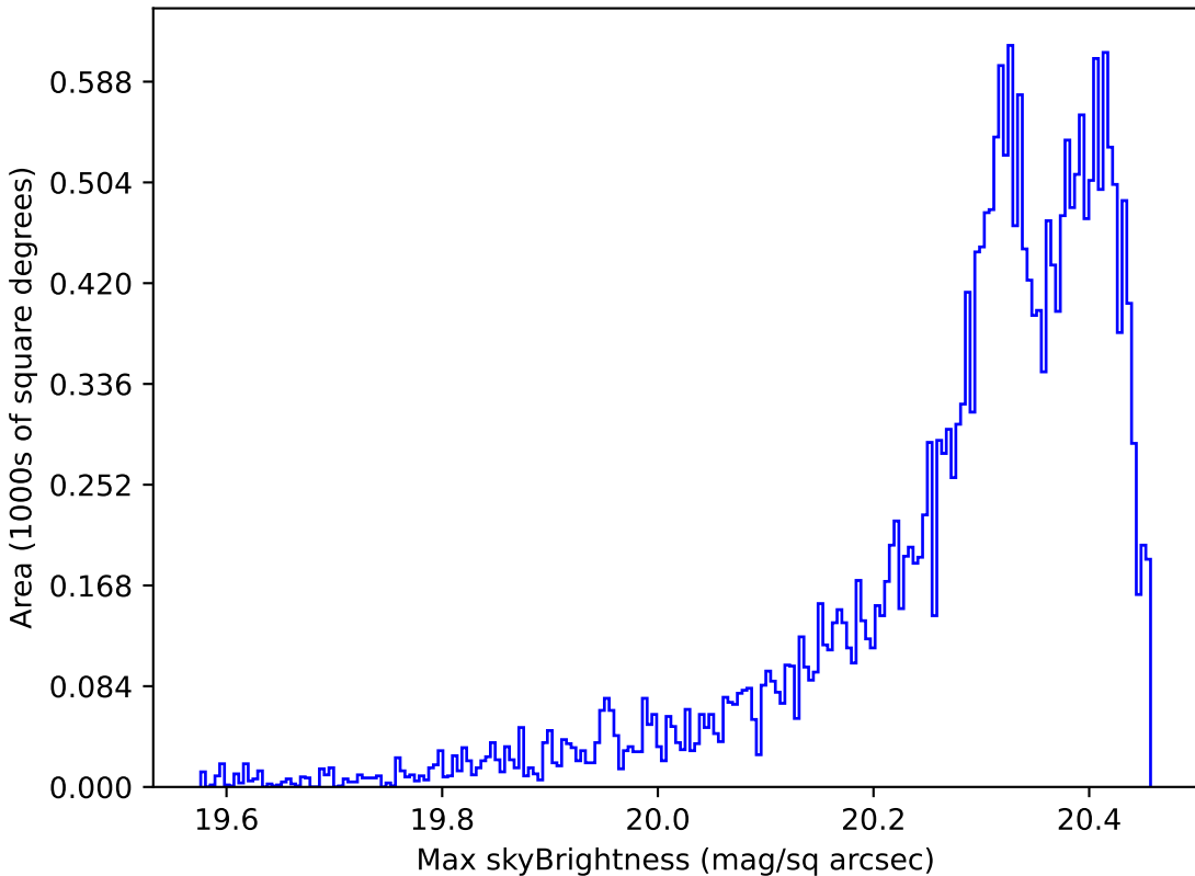
ddf_loaded_fl1_v3.4_10yrs Yr 1 i band: Max skyBrightness
