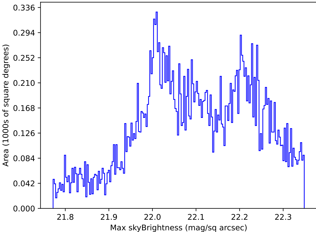
ddf_loaded_fl1_v3.4_10yrs Yr 1 g band: Max skyBrightness
