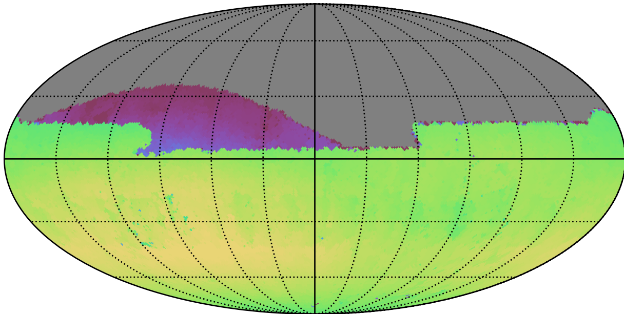
ddf_loaded_fl1_v3.4_10yrs Yr 1 all bands: Max skyBrightness
