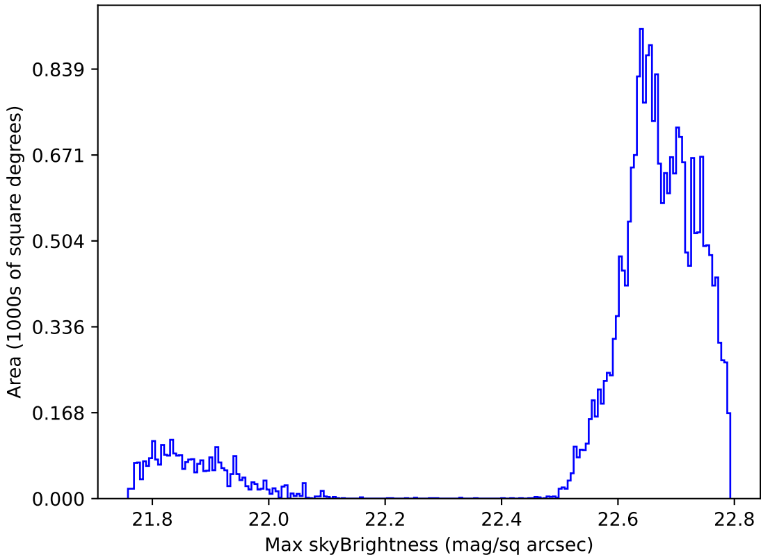
ddf_loaded_fl1_v3.4_10yrs Yr 1 all bands: Max skyBrightness
