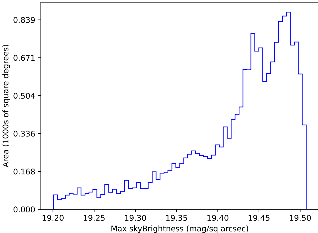
ddf_loaded_fl1_v3.4_10yrs WFD z band: Max skyBrightness
