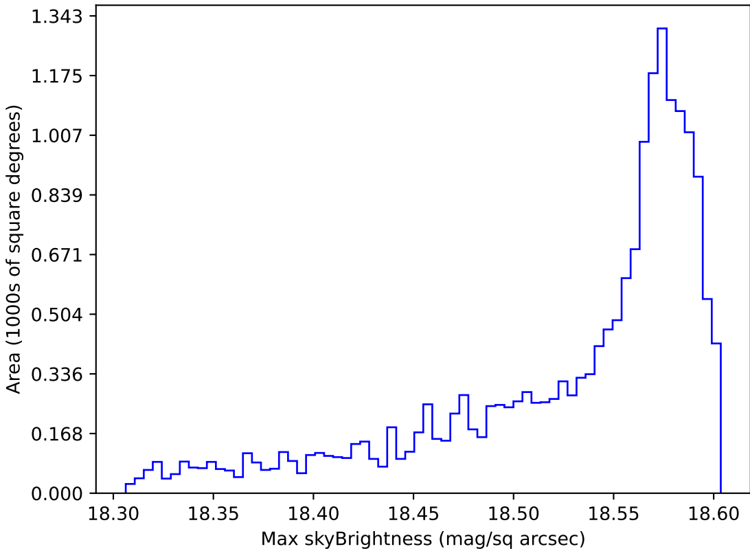
ddf_loaded_fl1_v3.4_10yrs WFD y band: Max skyBrightness
