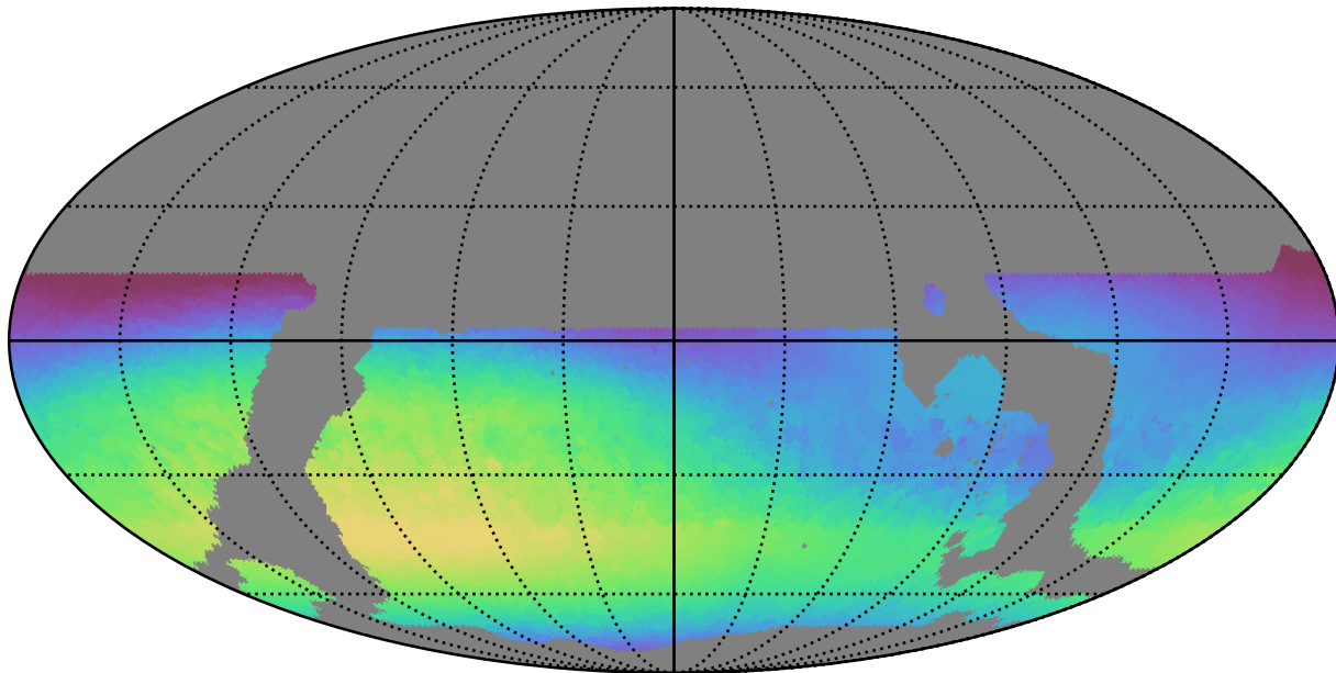
ddf_loaded_fl1_v3.4_10yrs WFD u band: Max skyBrightness
