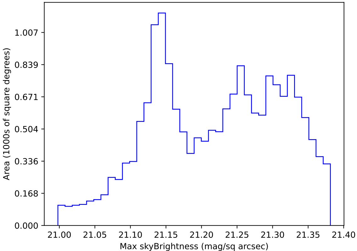
ddf_loaded_fl1_v3.4_10yrs WFD r band: Max skyBrightness
