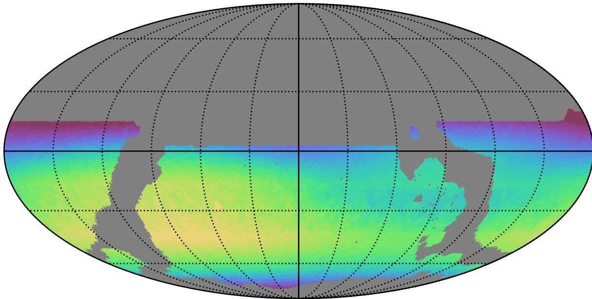
ddf_loaded_fl1_v3.4_10yrs WFD i band: Max skyBrightness
