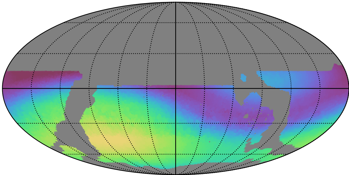
ddf_loaded_fl1_v3.4_10yrs WFD g band: Max skyBrightness
