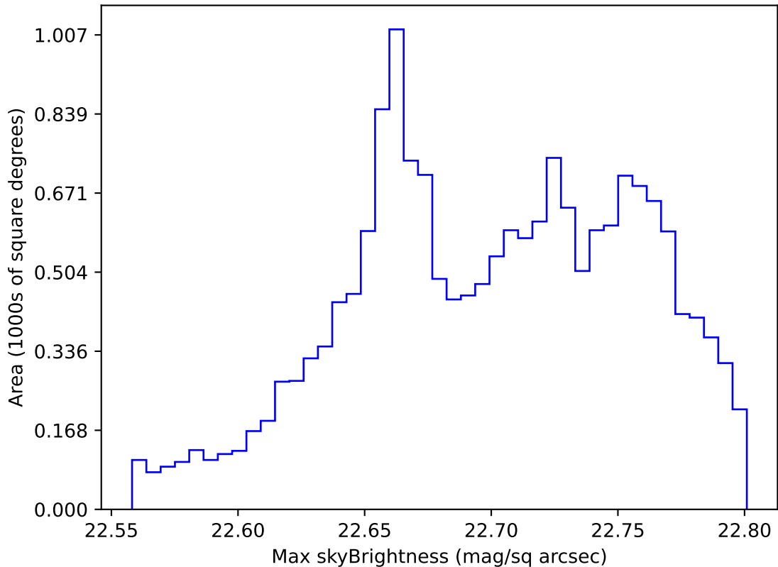
ddf_loaded_fl1_v3.4_10yrs WFD all bands: Max skyBrightness
