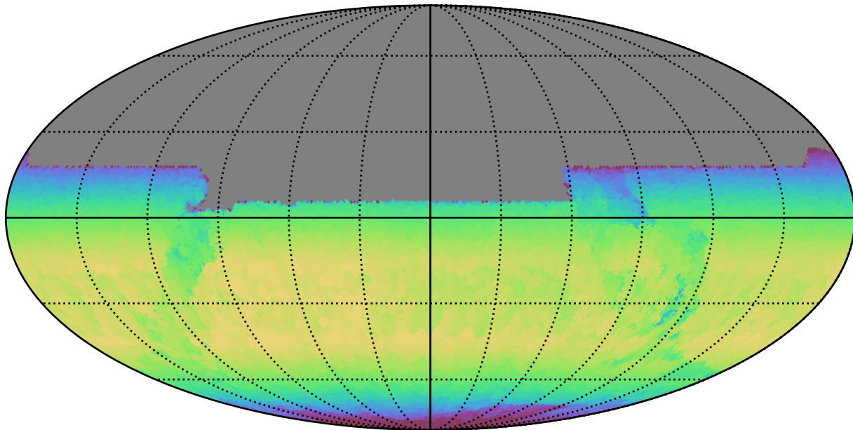
ddf_loaded_fl1_v3.4_10yrs All sky y band: Max skyBrightness
