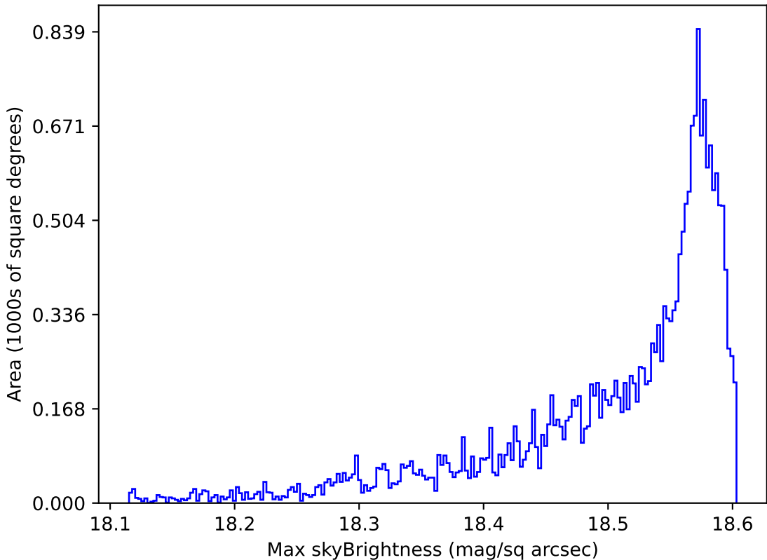
ddf_loaded_fl1_v3.4_10yrs All sky y band: Max skyBrightness
