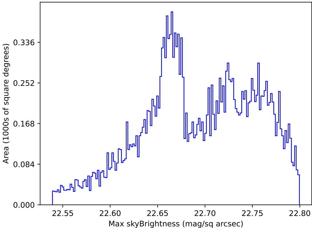
ddf_loaded_fl1_v3.4_10yrs All sky u band: Max skyBrightness
