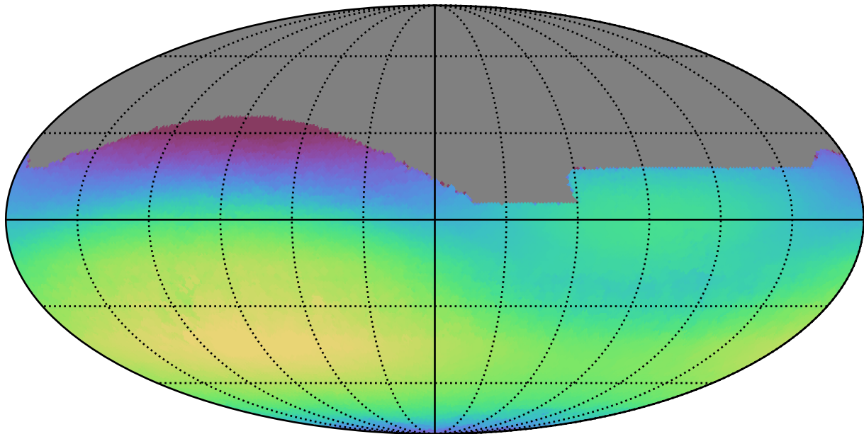
ddf_loaded_fl1_v3.4_10yrs All sky r band: Max skyBrightness
