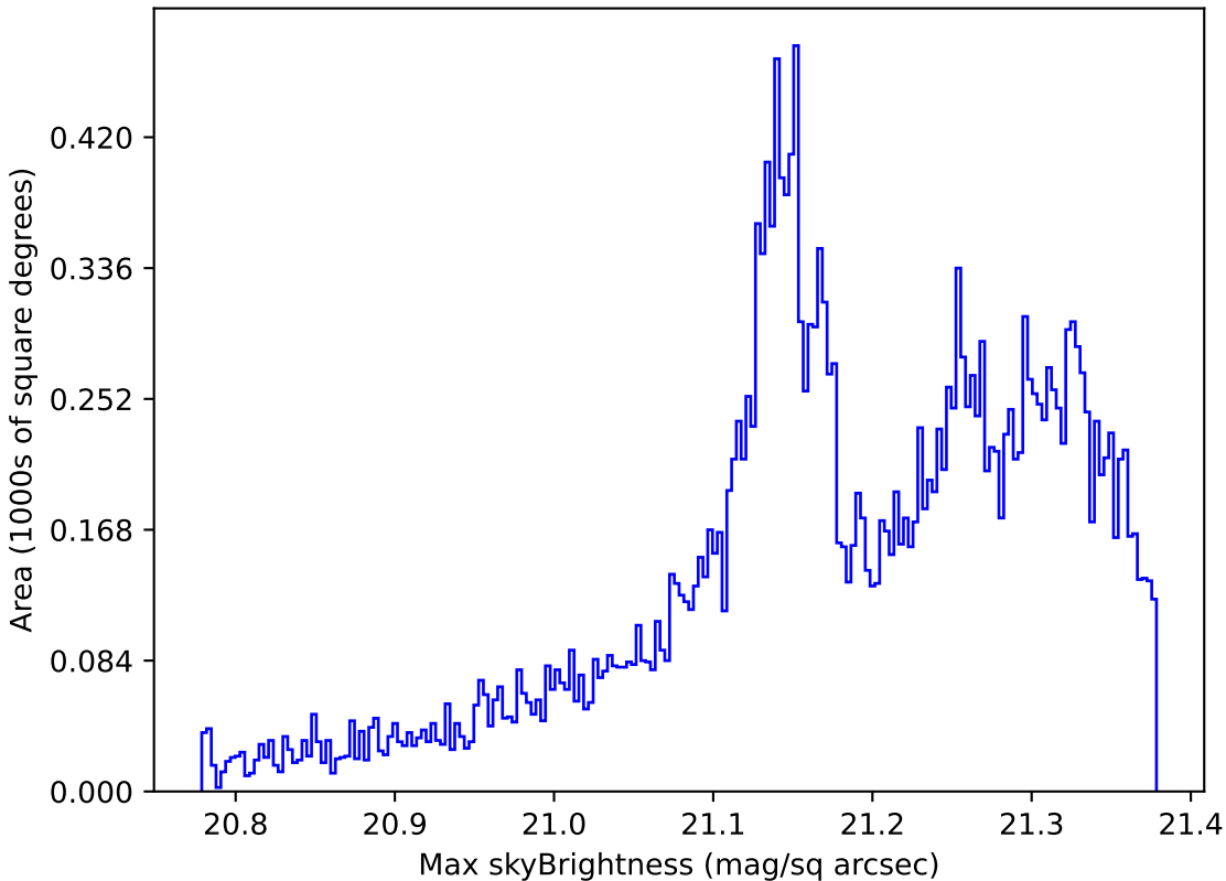
ddf_loaded_fl1_v3.4_10yrs All sky r band: Max skyBrightness
