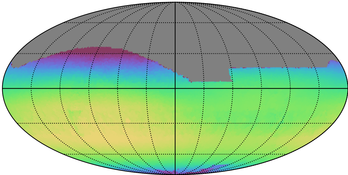
ddf_loaded_fl1_v3.4_10yrs All sky i band: Max skyBrightness
