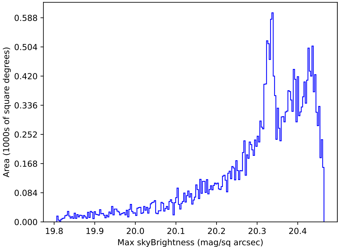
ddf_loaded_fl1_v3.4_10yrs All sky i band: Max skyBrightness
