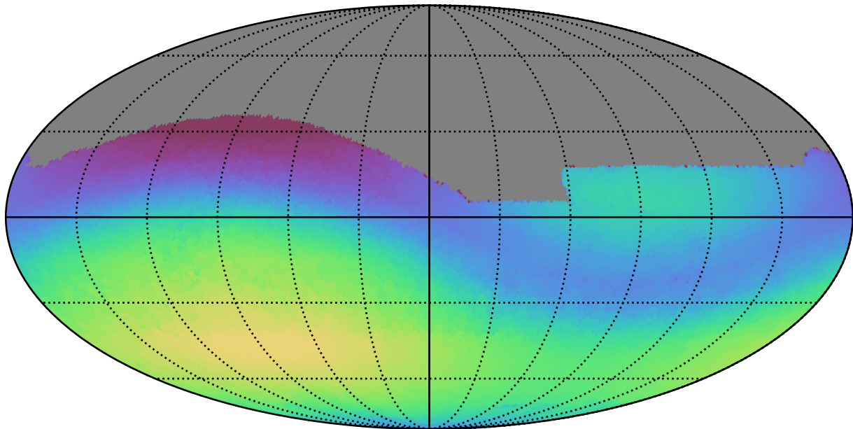
ddf_loaded_fl1_v3.4_10yrs All sky g band: Max skyBrightness
