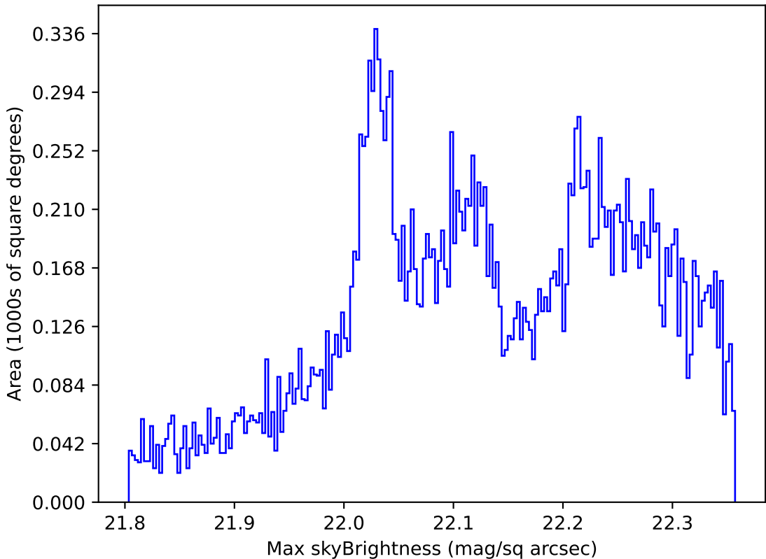
ddf_loaded_fl1_v3.4_10yrs All sky g band: Max skyBrightness
