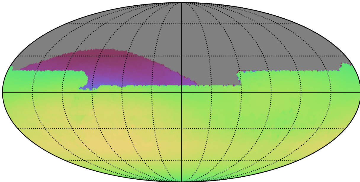
ddf_loaded_fl1_v3.4_10yrs All sky all bands: Max skyBrightness
