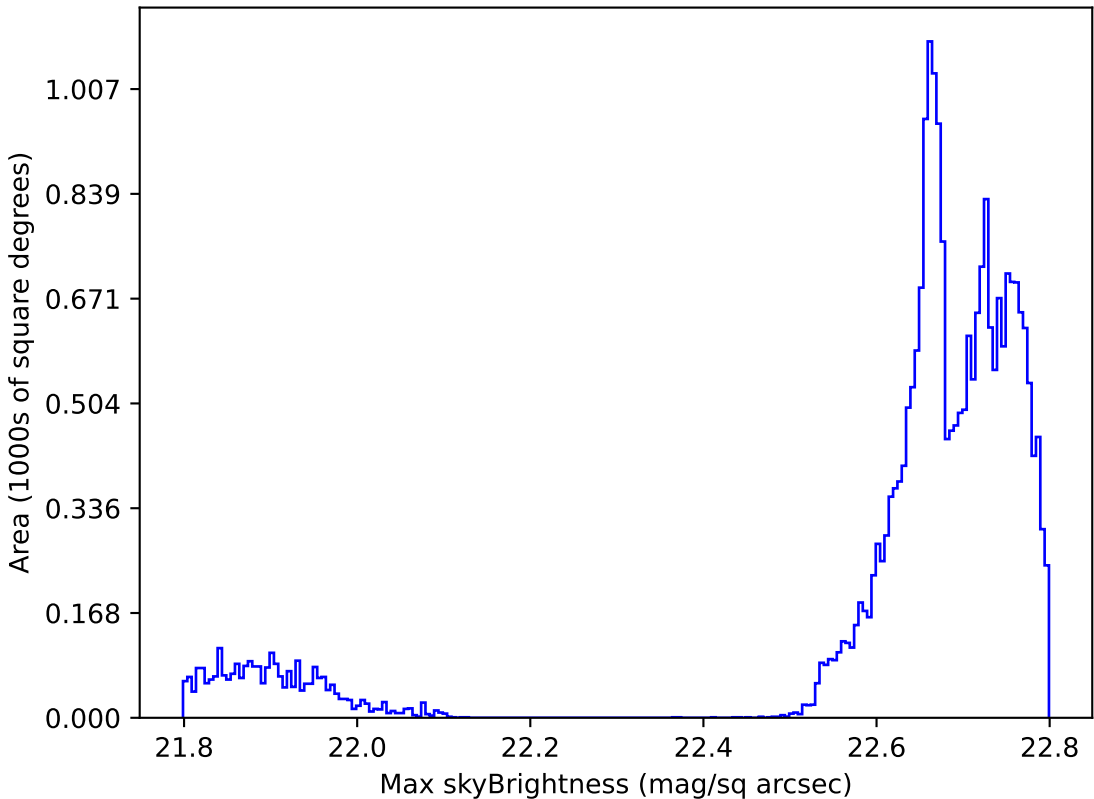
ddf_loaded_fl1_v3.4_10yrs All sky all bands: Max skyBrightness
