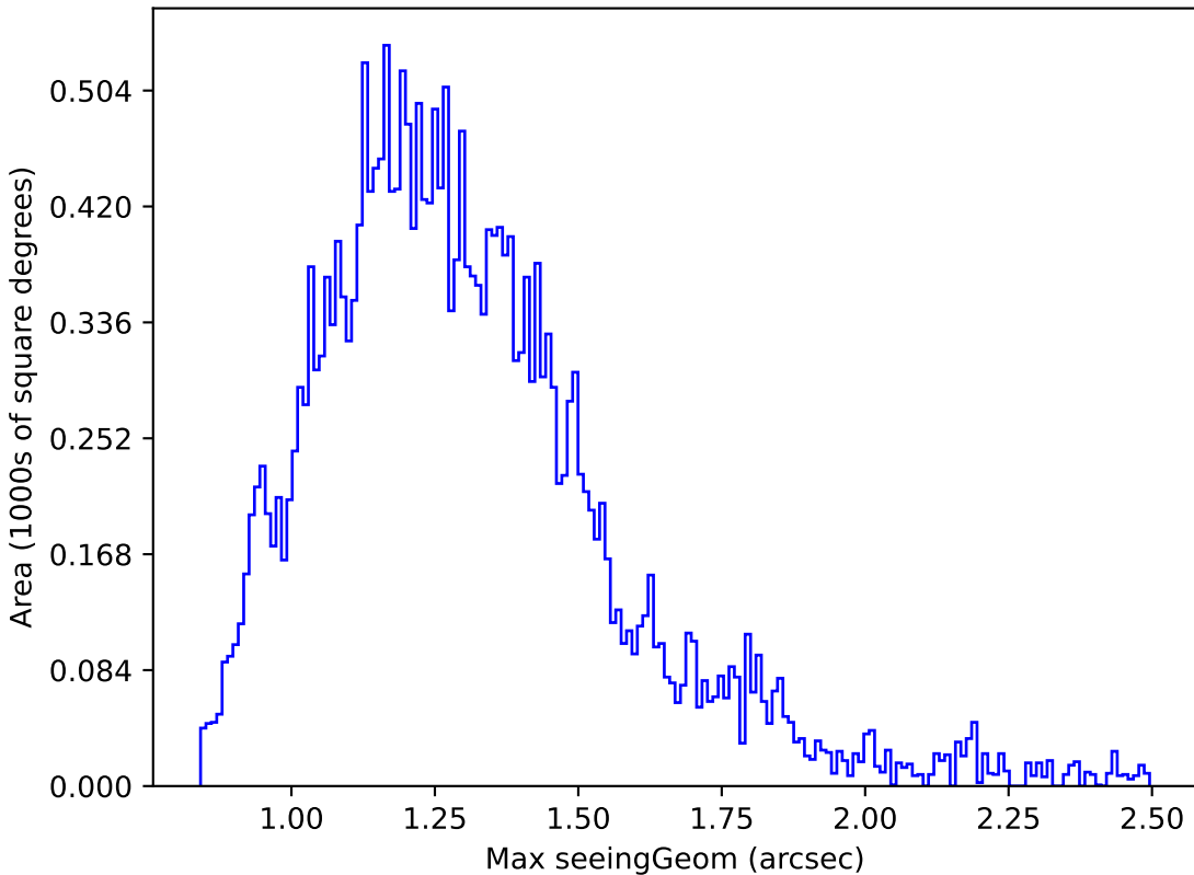
ddf_loaded_fl1_v3.4_10yrs Yr 1 z band: Max seeingGeom
