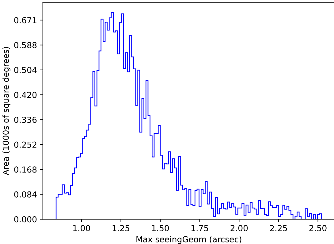
ddf_loaded_fl1_v3.4_10yrs Yr 1 y band: Max seeingGeom
