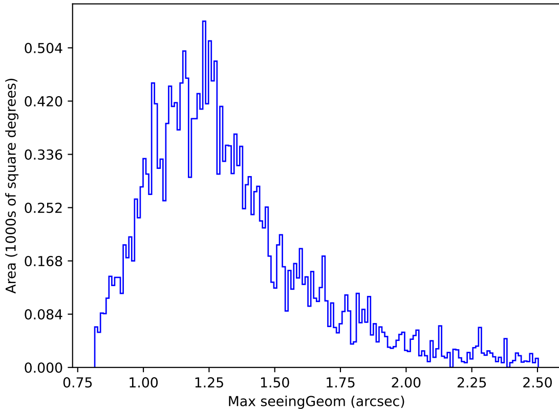
ddf_loaded_fl1_v3.4_10yrs Yr 1 u band: Max seeingGeom
