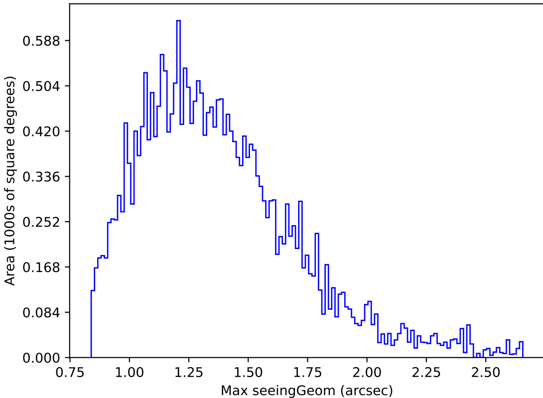
ddf_loaded_fl1_v3.4_10yrs Yr 1 r band: Max seeingGeom
