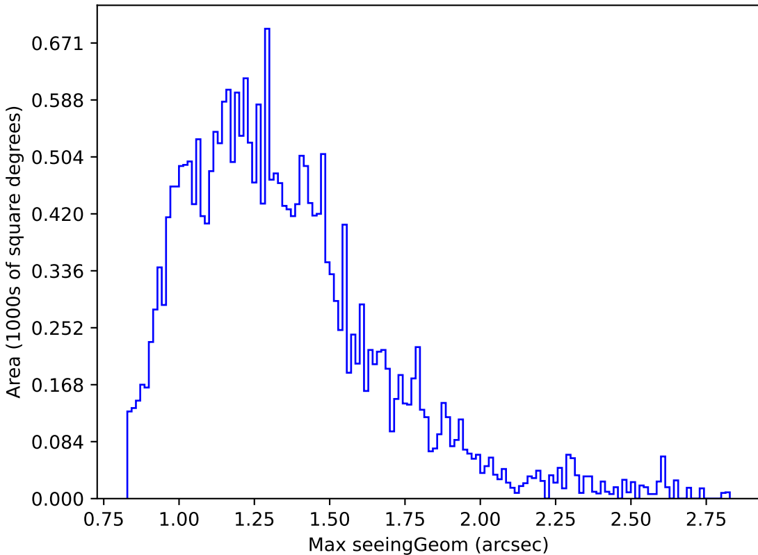
ddf_loaded_fl1_v3.4_10yrs Yr 1 i band: Max seeingGeom
