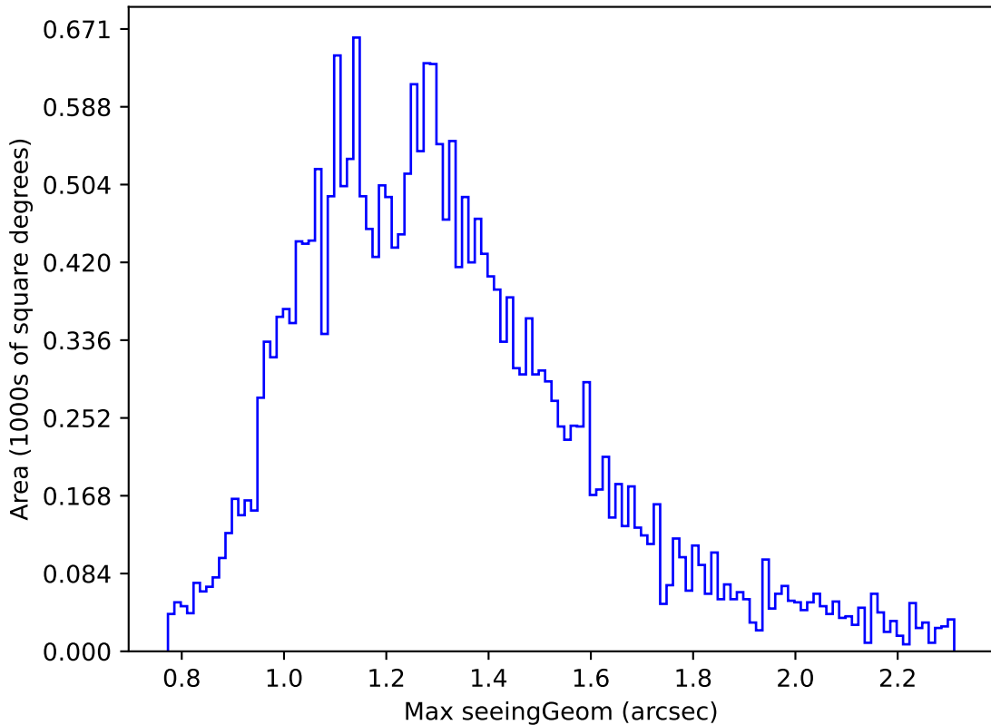
ddf_loaded_fl1_v3.4_10yrs Yr 1 g band: Max seeingGeom
