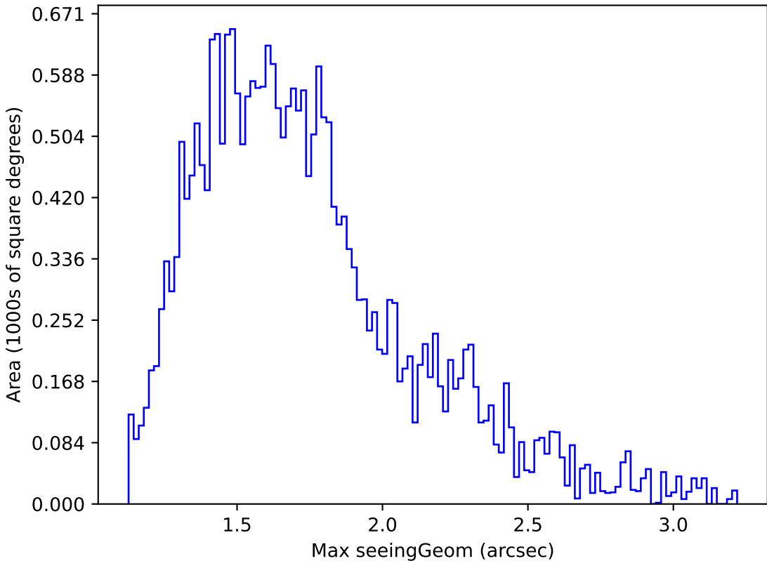
ddf_loaded_fl1_v3.4_10yrs Yr 1 all bands: Max seeingGeom
