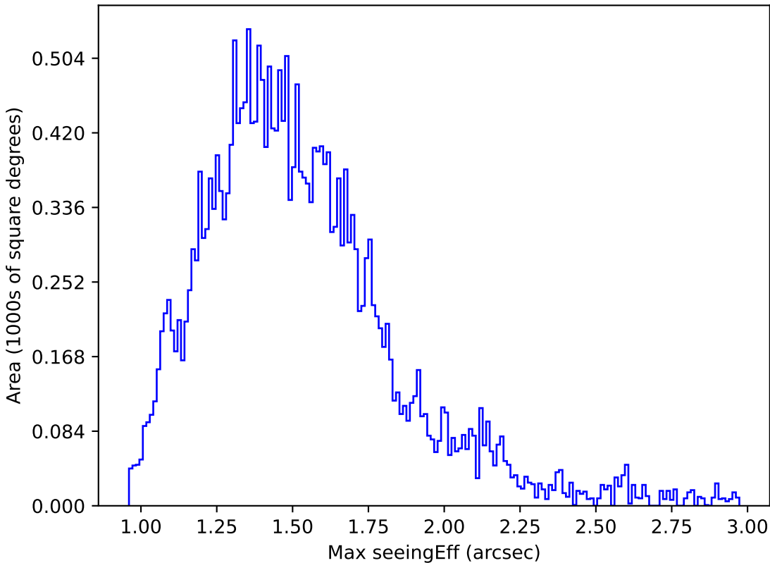
ddf_loaded_fl1_v3.4_10yrs Yr 1 z band: Max seeingEff
