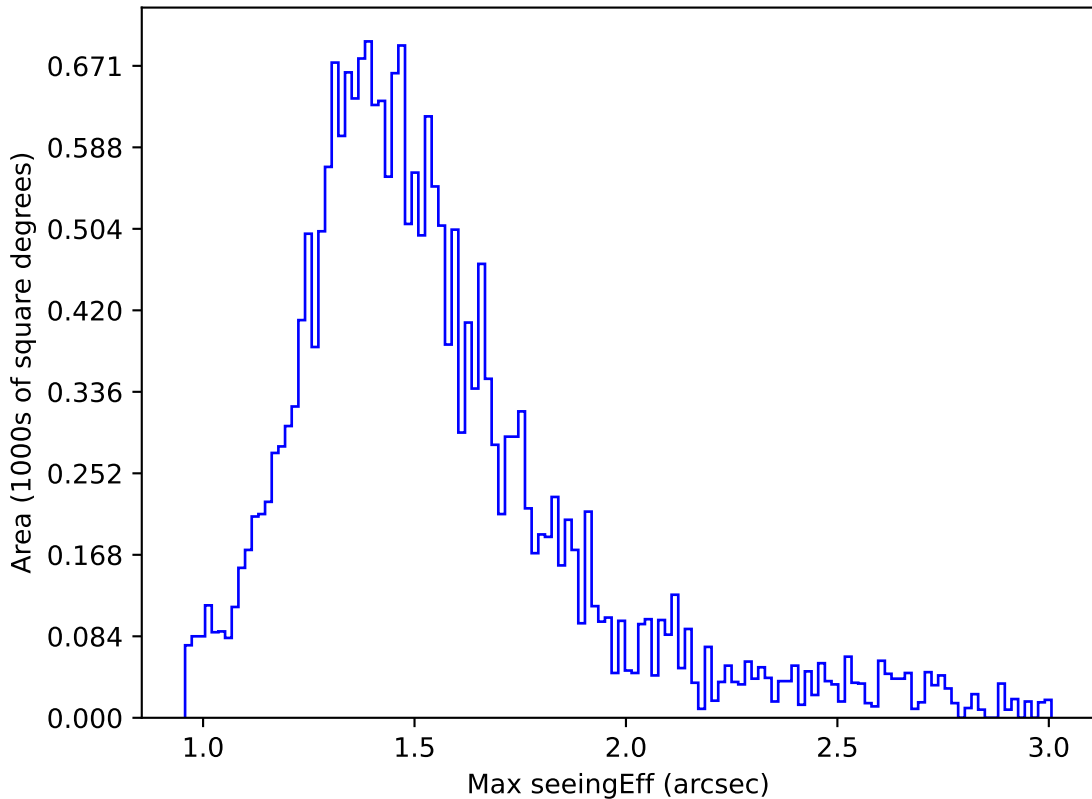
ddf_loaded_fl1_v3.4_10yrs Yr 1 y band: Max seeingEff
