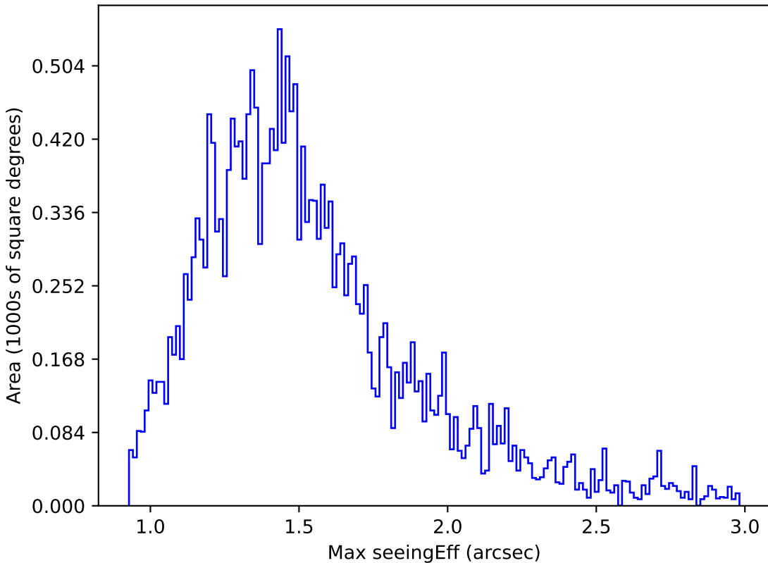
ddf_loaded_fl1_v3.4_10yrs Yr 1 u band: Max seeingEff
