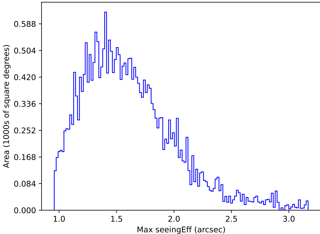
ddf_loaded_fl1_v3.4_10yrs Yr 1 r band: Max seeingEff
