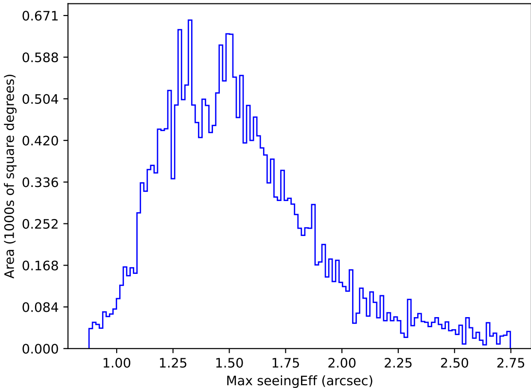
ddf_loaded_fl1_v3.4_10yrs Yr 1 g band: Max seeingEff
