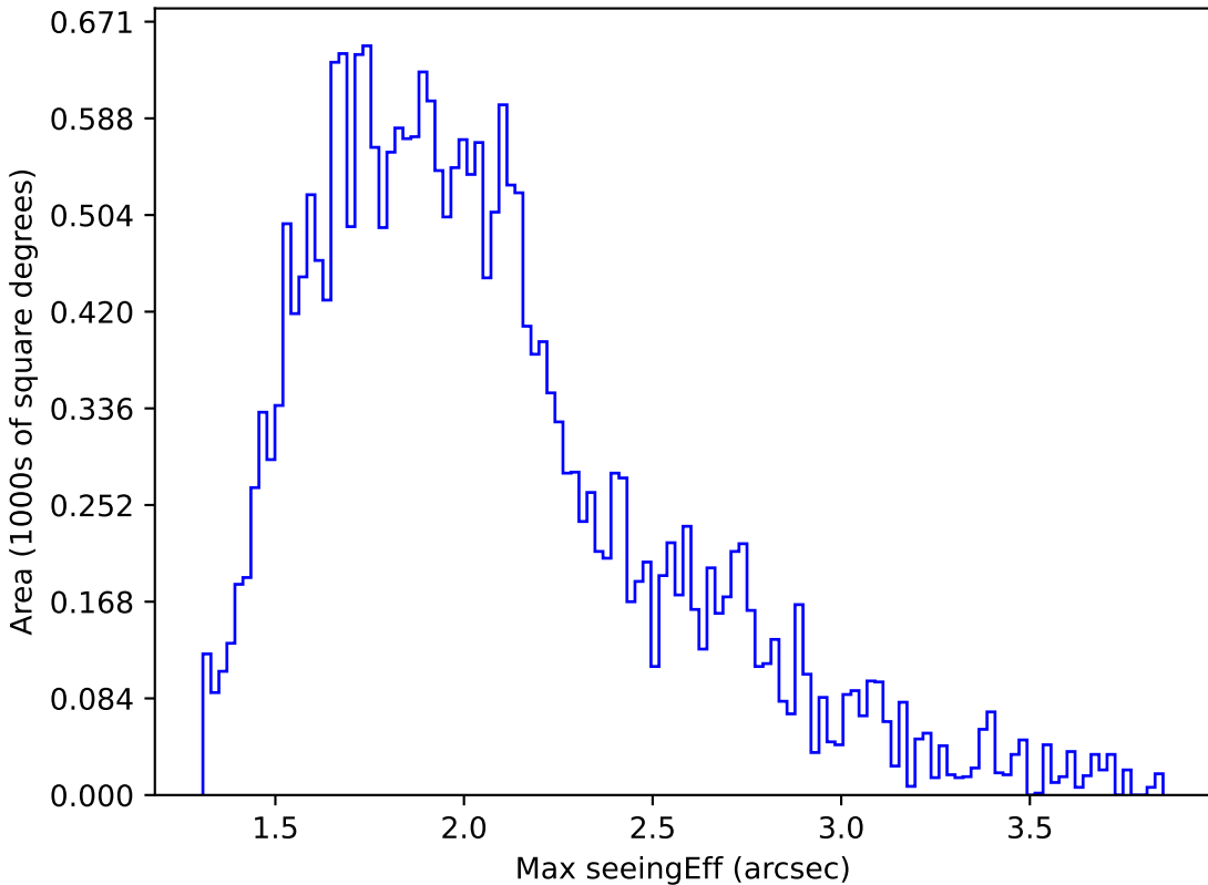
ddf_loaded_fl1_v3.4_10yrs Yr 1 all bands: Max seeingEff
