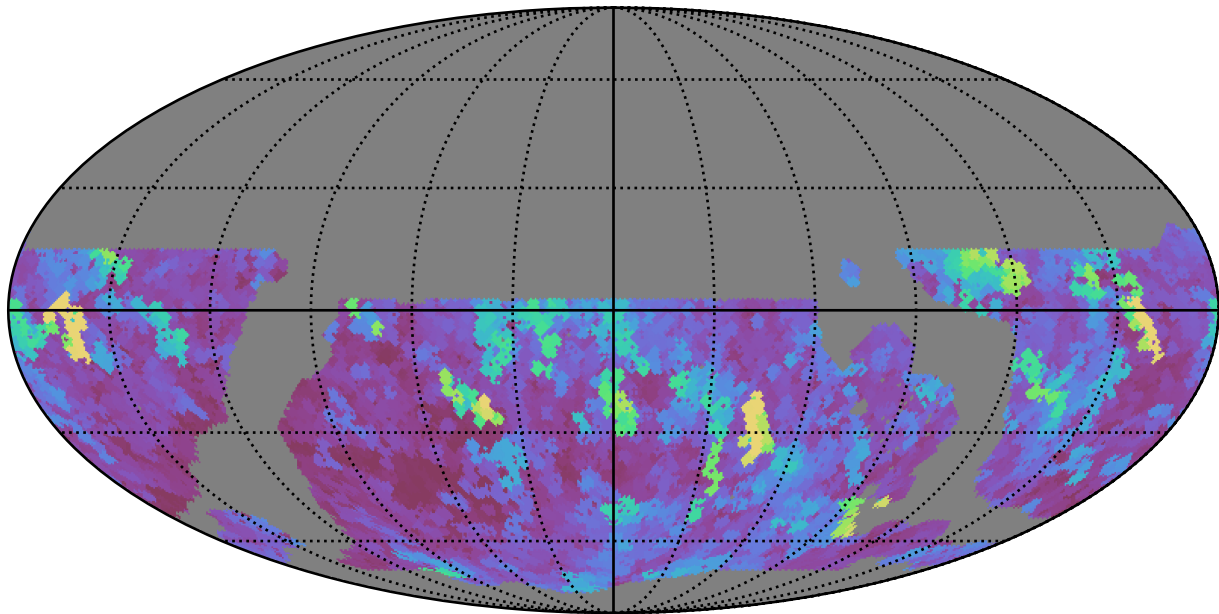
ddf_loaded_fl1_v3.4_10yrs WFD z band: Max seeingEff
