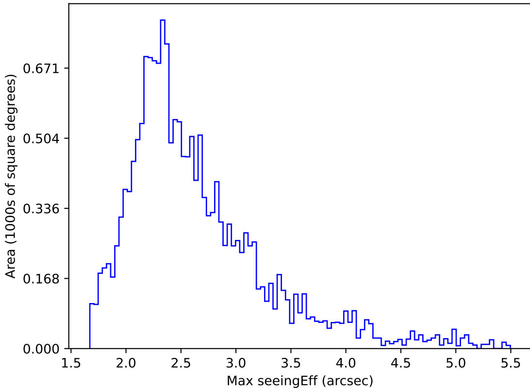
ddf_loaded_fl1_v3.4_10yrs WFD z band: Max seeingEff
