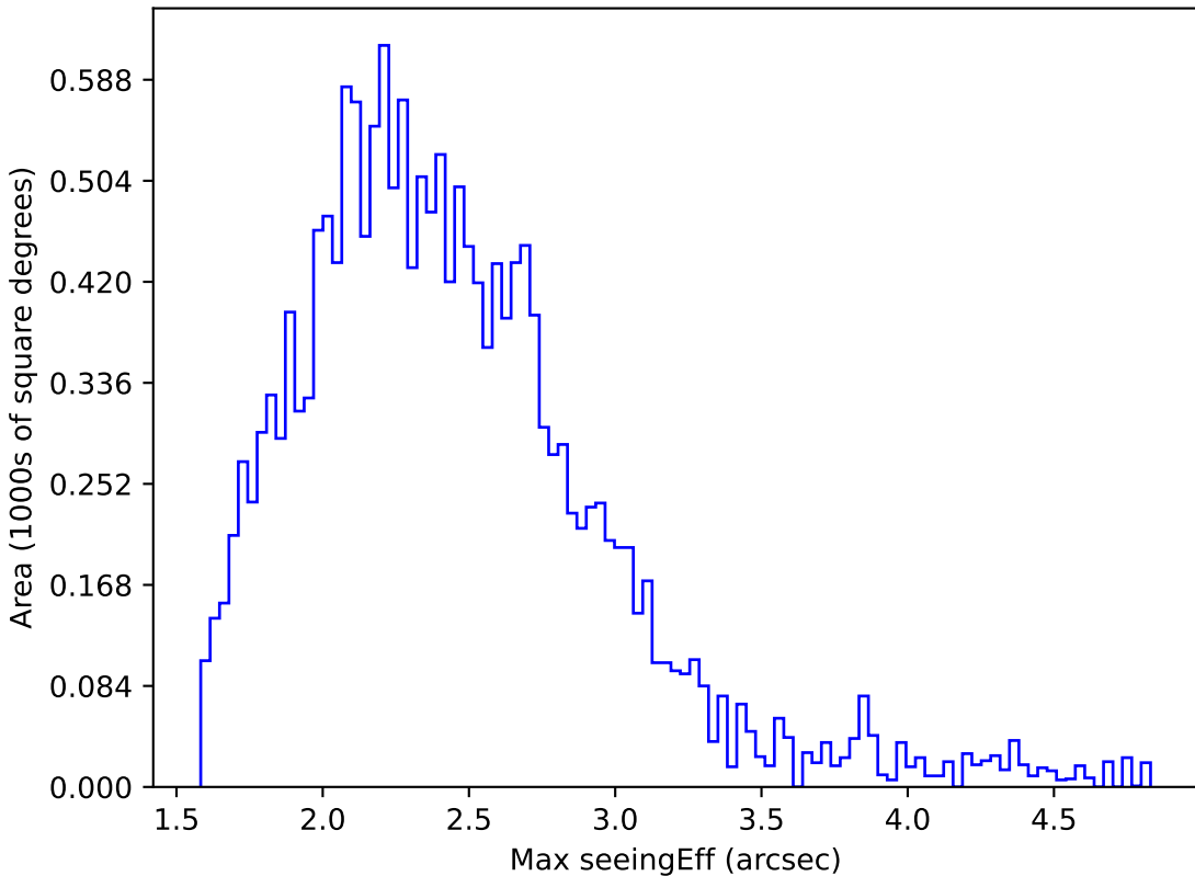
ddf_loaded_fl1_v3.4_10yrs WFD y band: Max seeingEff
