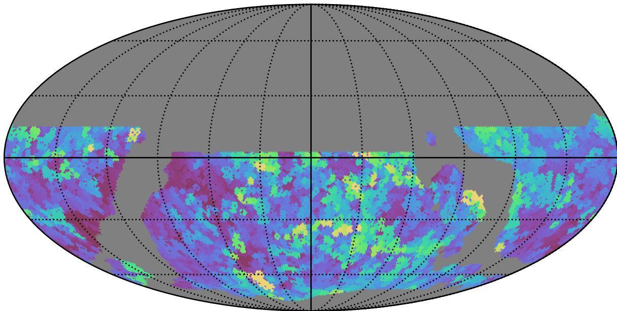
ddf_loaded_fl1_v3.4_10yrs WFD u band: Max seeingEff
