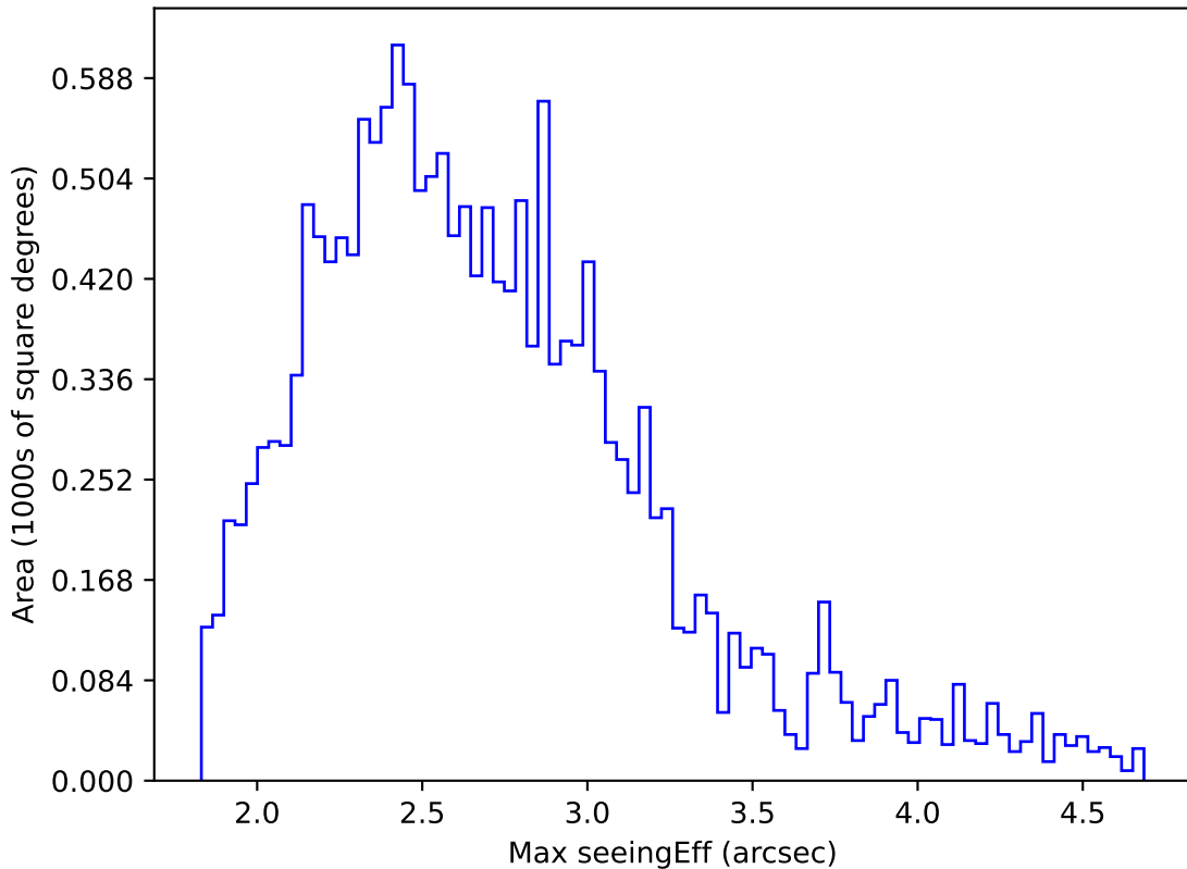
ddf_loaded_fl1_v3.4_10yrs WFD r band: Max seeingEff
