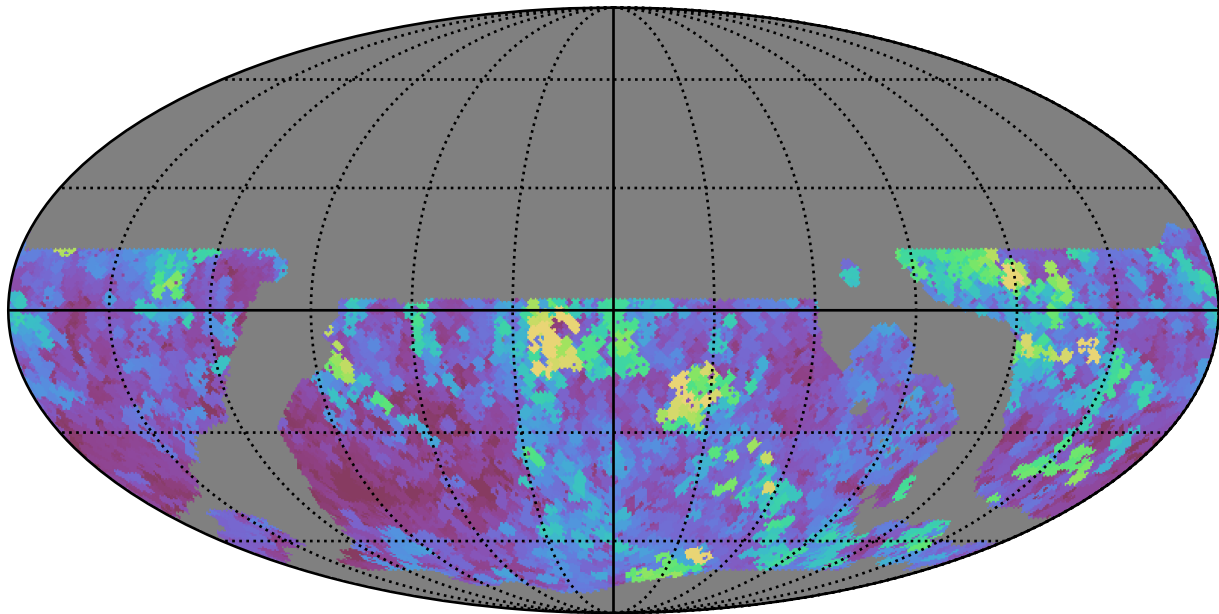
ddf_loaded_fl1_v3.4_10yrs WFD i band: Max seeingEff
