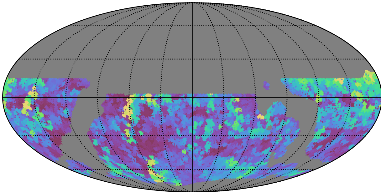
ddf_loaded_fl1_v3.4_10yrs WFD g band: Max seeingEff
