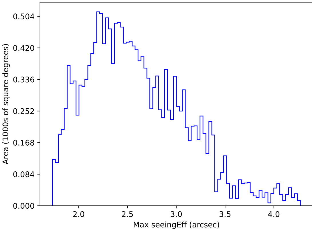
ddf_loaded_fl1_v3.4_10yrs WFD g band: Max seeingEff
