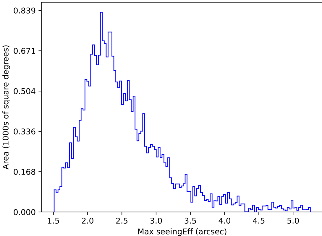
ddf_loaded_fl1_v3.4_10yrs All sky z band: Max seeingEff
