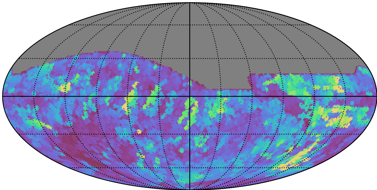
ddf_loaded_fl1_v3.4_10yrs All sky r band: Max seeingEff
